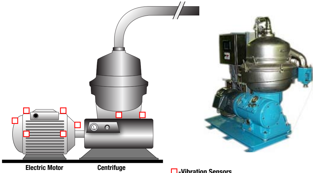
□ -Vibration Sensors
