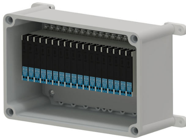
IS211 11-20 Intrinsically Safe Barriers with Enclosure
